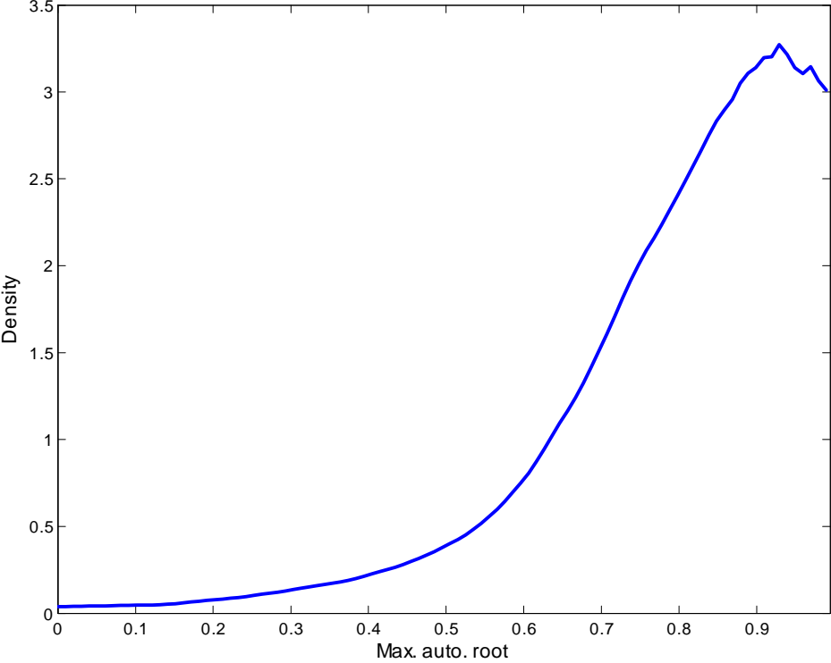
Figure 4: Max autoregressive roots.
