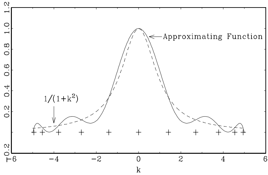
Function Approximation with Chebychev Zeros
