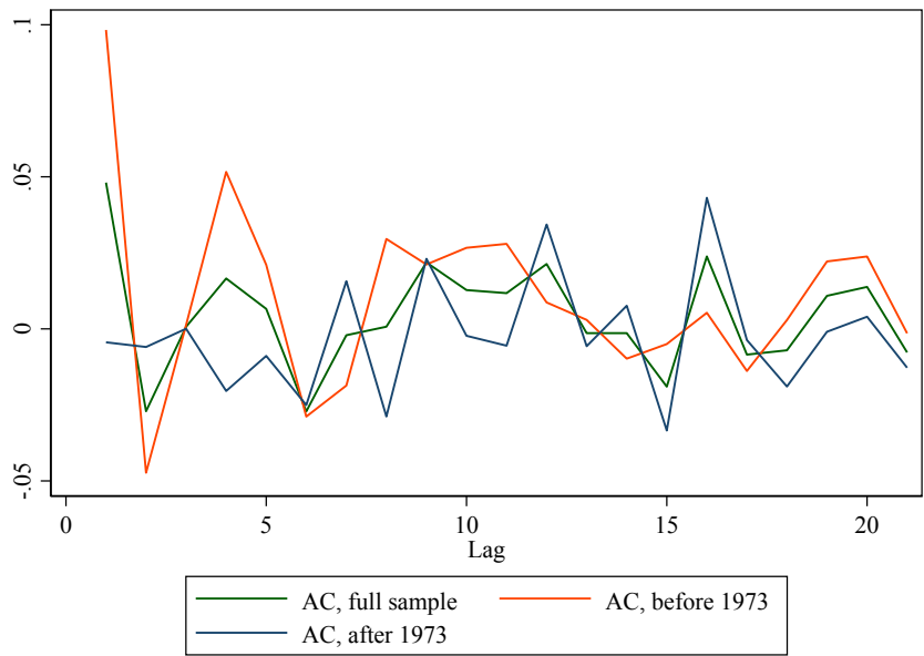
(a) Autocorrelations
