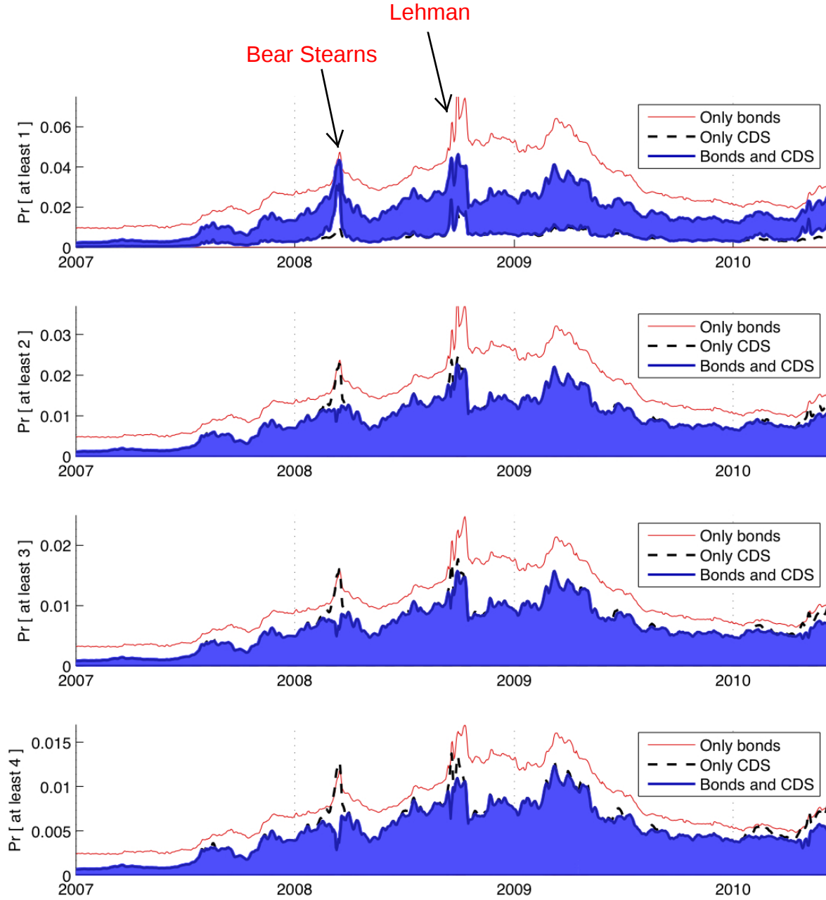
Figure 4: Upper and lower bounds on different systemic events under the assumption of nonnegative liquidity premia: average monthly probability of at least r banks defaulting, for r = 1, 2, 3, 4 . The Figure reports bounds obtained using only information in bond prices (thin lines), only CDS spreads (dotted lines), and all information (shaded area). To reduce noise, I plot a 3 day moving average of each bound. Note that all lower bounds are 0 for r > 1 , and that the CDS-only bounds often coincide with the full information bounds (that use both bonds and CDSs).
