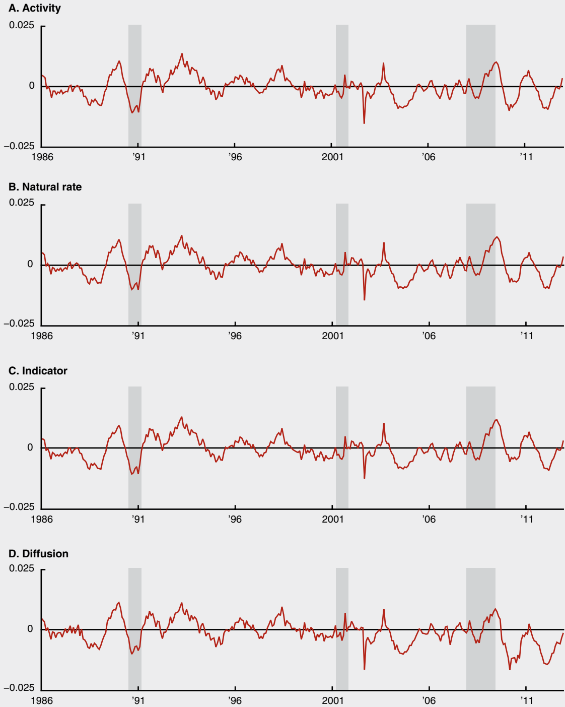
Errors from 12-month-ahead PCE forecast, 1985–2007 coefficients
